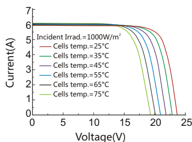
Current-Voltage Curve
