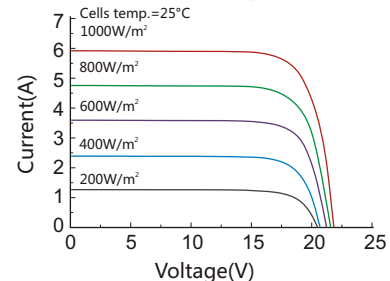
Current-Voltage Curve
